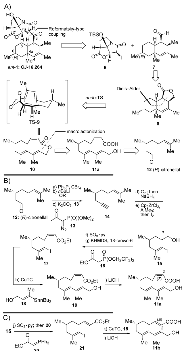
Scheme 1. A) Retrosynthetic analysis for ent -CJ-16,264 ( ent -1) and synthesis of ( Z )- and ( E )-hydroxy acids 11a and 11b . B) Reagents and conditions: a) \text{CBr}_4 (2.0 equiv), \text{PPh}_3 (4.0 equiv), \text{CH}_2\text{Cl}_2 , 0^\circ\text{C} , 3 h, 98%; b) n\text{BuLi} (3.0 equiv), THF, -78^\circ\text{C} , 2 h, 95%; c) \text{K}_2\text{CO}_3 , 13 , MeOH, 25^\circ\text{C} , 10 h, 85%; d) \text{O}_3 , \text{CH}_2\text{Cl}_2 :MeOH (1:1), -78^\circ\text{C} , 2 h; then \text{NaBH}_4 (1.1 equiv), -78 \rightarrow 25^\circ\text{C} , 4 h, 85%; e) \text{Cp}_2\text{ZrCl}_2 (1.1 equiv), \text{AlMe}_3 (4.0 equiv), \text{ClCH}_2\text{CH}_2\text{Cl} , 25^\circ\text{C} , 5 h; then \text{I}_2 , THF, -20^\circ\text{C} , 2 h, 84%; f) \text{SO}_3 \cdot \text{py} (2.0 equiv), \text{Et}_3\text{N} (4.0 equiv), \text{CH}_2\text{Cl}_2 :DMSO (3:1), 0^\circ\text{C} , 1 h, 91%; g) \text{LiHMDS} (1.2 equiv), 18-crown-6 (5.0 equiv), 16 (1.2 equiv), THF, 0^\circ\text{C} , 2 h, 92% ( \geq 95\% Z:E d.r.); h) \text{CuTC} (6.0 equiv), 18 (3.0 equiv), DMF, 0 \rightarrow 25^\circ\text{C} , 2 h, 85%; i) \text{LiOH} (35.0 equiv), THF:H _2\text{O} (1:1), 60^\circ\text{C} , 18 h, 99%. C) Reagents and conditions: j) \text{SO}_3 \cdot \text{py} (2.0 equiv), \text{Et}_3\text{N} (4.0 equiv), \text{CH}_2\text{Cl}_2 :DMSO (3:1), 0^\circ\text{C} , 1 h; then 20 , 25^\circ\text{C} , 4 h, 90%; k) \text{CuTC} (6.0 equiv), 18 (3.0 equiv), DMF, 0 \rightarrow 25^\circ\text{C} , 2 h, 88%; l) \text{LiOH} (35.0 equiv), THF:H _2\text{O} (1:1), 60^\circ\text{C} , 20 h, 99%. Abbreviations: TBS = tert -butyldimethylsilyl; Cp = cyclopentadienyl; LiHMDS = lithium bis(trimethylsilyl)amide; CuTC = copper(I)-thiophene-2-carboxylate.
